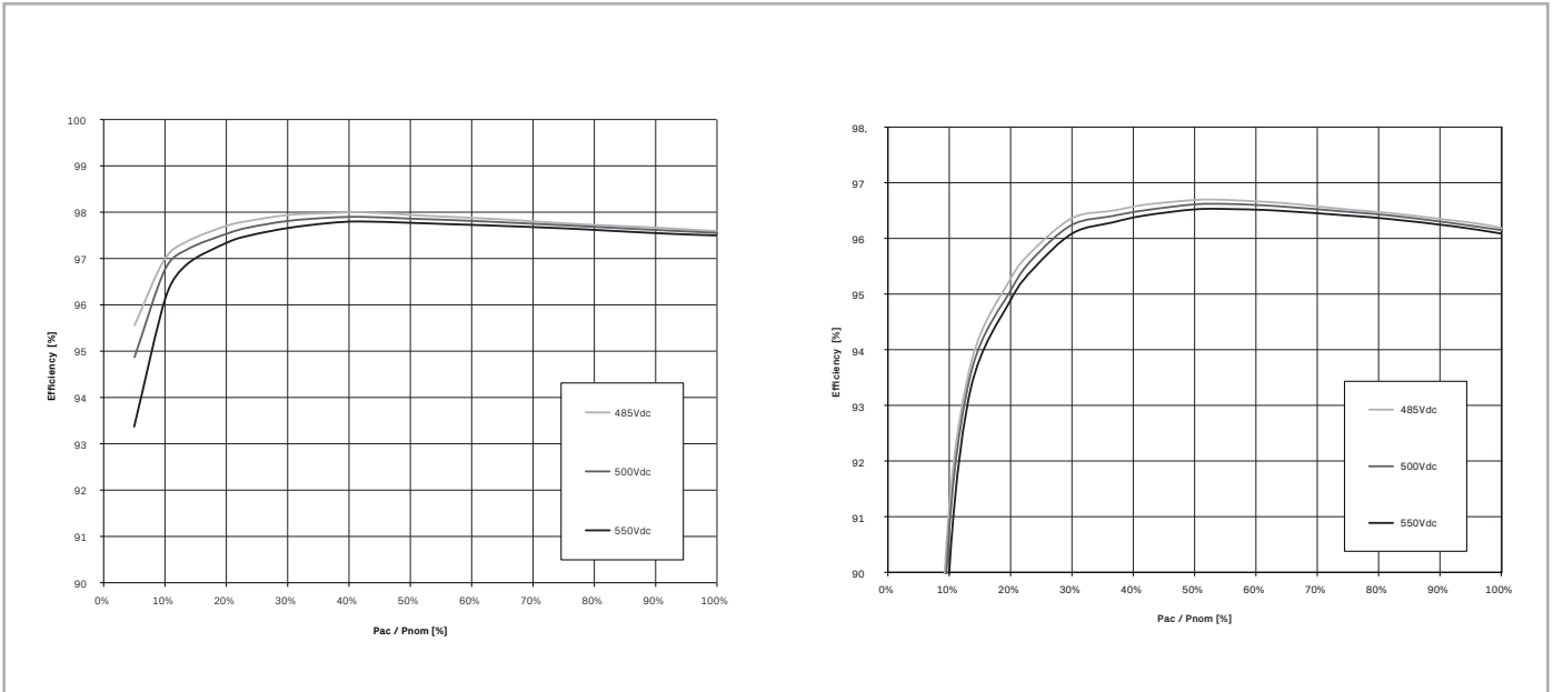
Efficiency curves PVI-55.0/330.0-TL
